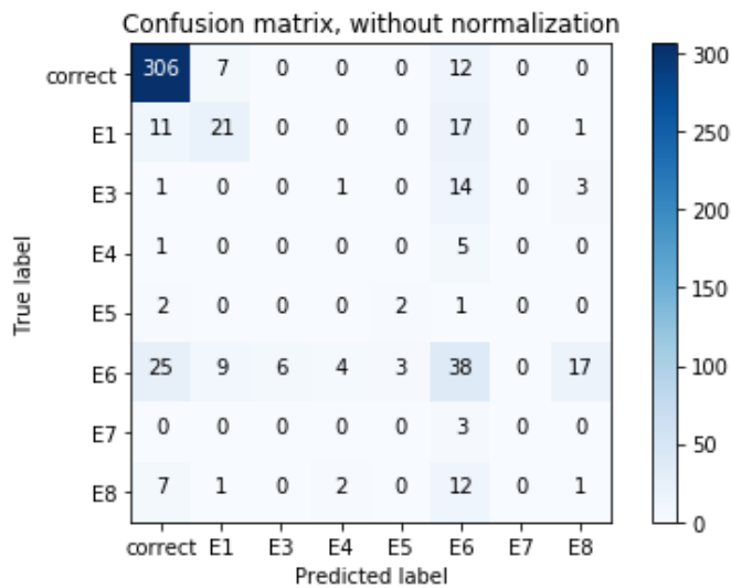
Fig. 7. Confusion matrix without normalization for multi-class XGBoost.
